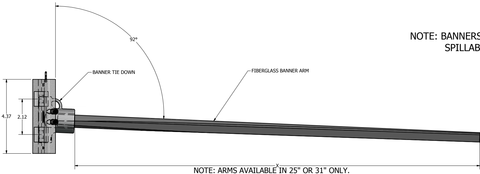
BANNER ARM CASTING DETAIL VIEW
