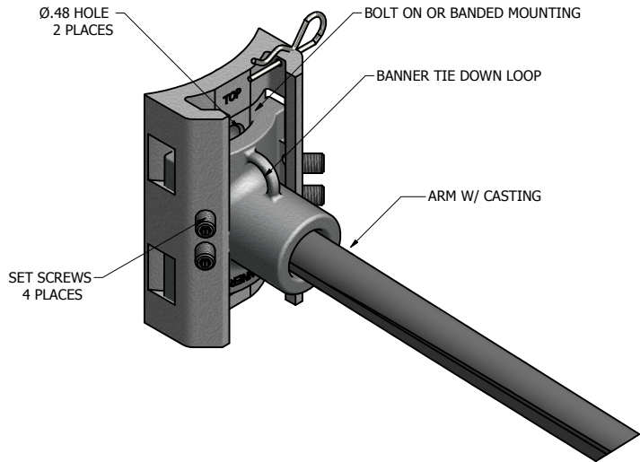
BANNER ARM CASTING DETAIL VIEW
